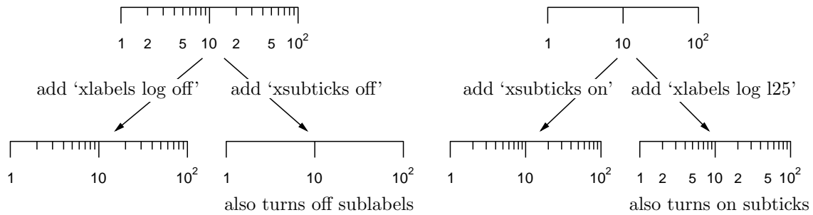
Figure 4.10: How log subticks and log sublabels interact.
