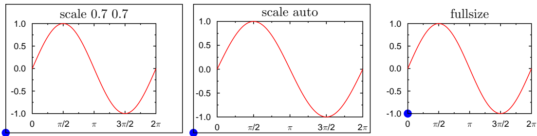
Figure 4.8: Different axis scaling options: default, automatic, and ‘fullsize’. The blue dot indicates the origin (x, y) of the graph, that is, the graph is generated with ‘ amove x y ’ followed by ‘ begin graph ’ ... ‘ end graph ’. The xaxis is labeled using the option ‘ format pi ’.
