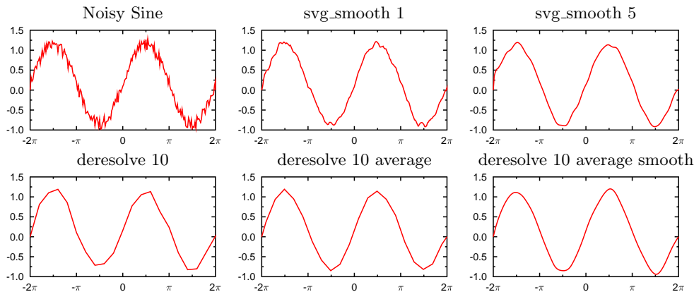
Figure 4.3: Various smooth options.
