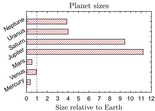
Figure 4.12: Illustration of the ‘horiz’ and ‘pattern’ keywords of the ‘bar’ command, and of the ‘angle’ option of the ‘yaxis’ command.
