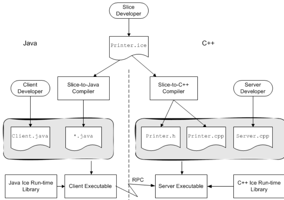
Development process for different development environments.
