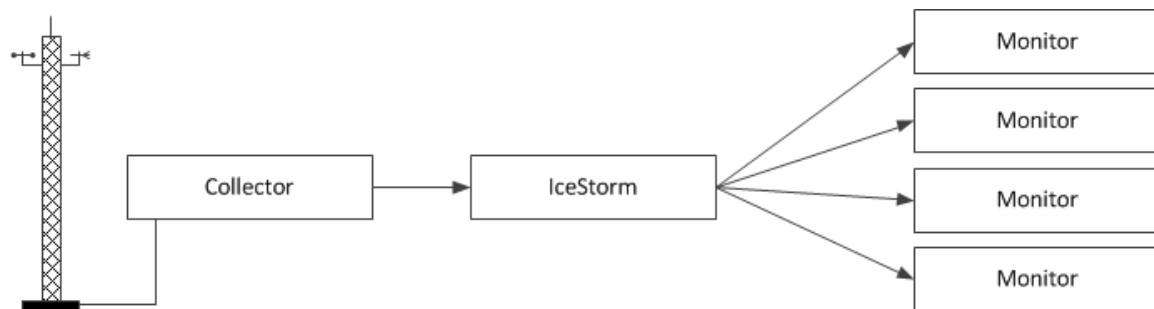
A weather monitoring application using IceStorm.
