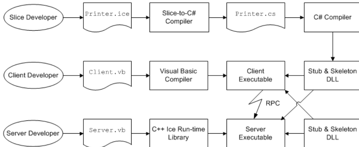
Developing a Visual Basic application with Ice.
