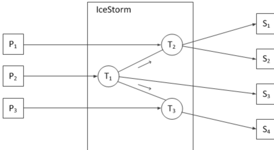
Topic federation.
