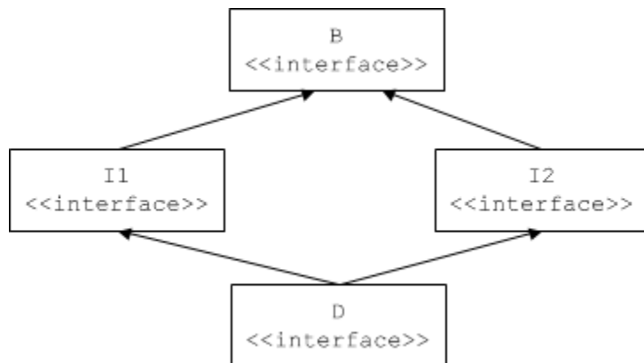
Diamond-shaped inheritance.
