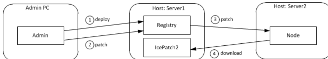
Overview of application distribution.
