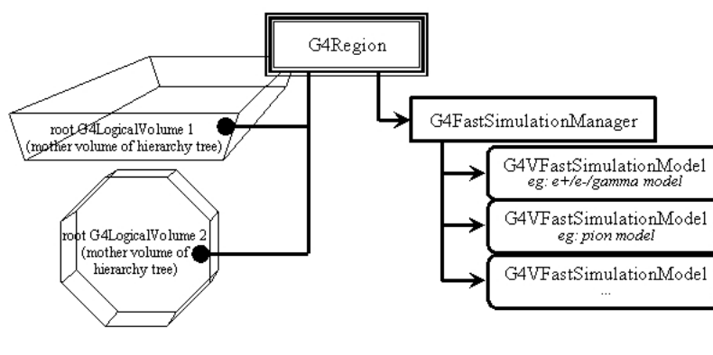
Fig. 5.3: G4VFastSimulationModel and G4FastSimulationManager objects.
