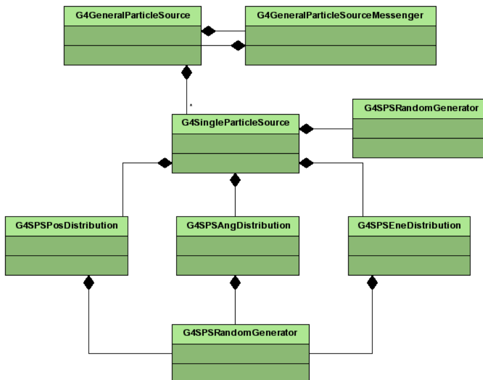
Figure 2.1. The class diagram of G4GeneralParticleSource .
