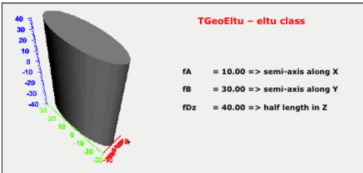
Figure 18.14: TGeoEltu Class
