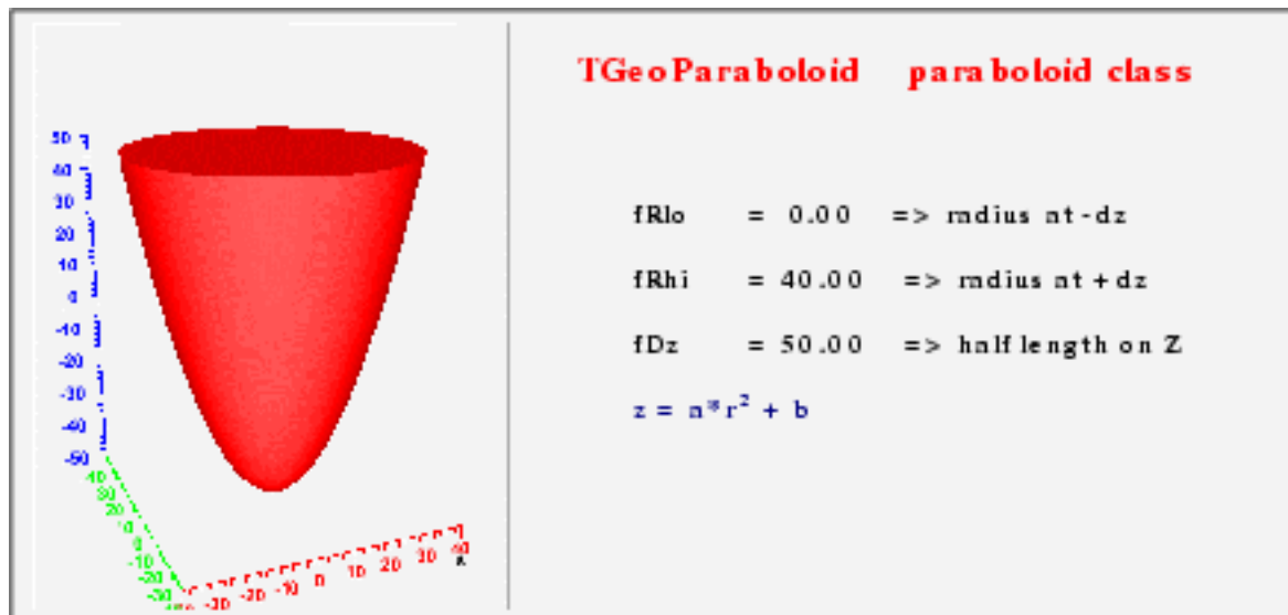
Figure 18.20: TGeoParaboloid Class
