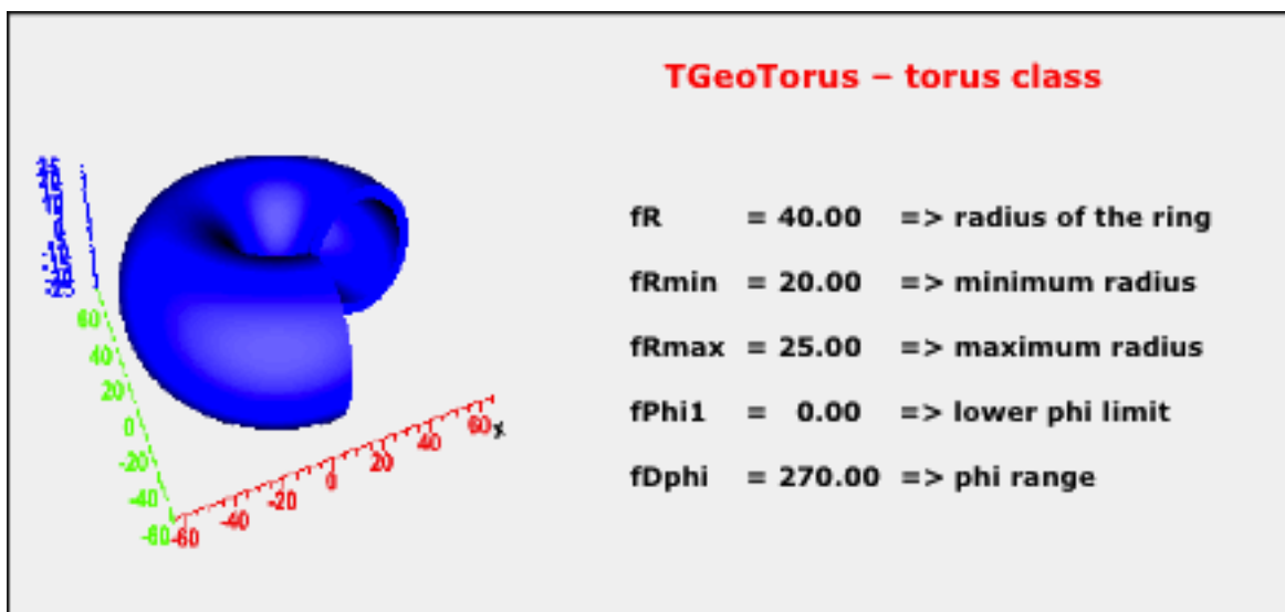
Figure 18.19: TGeoTorus Class
