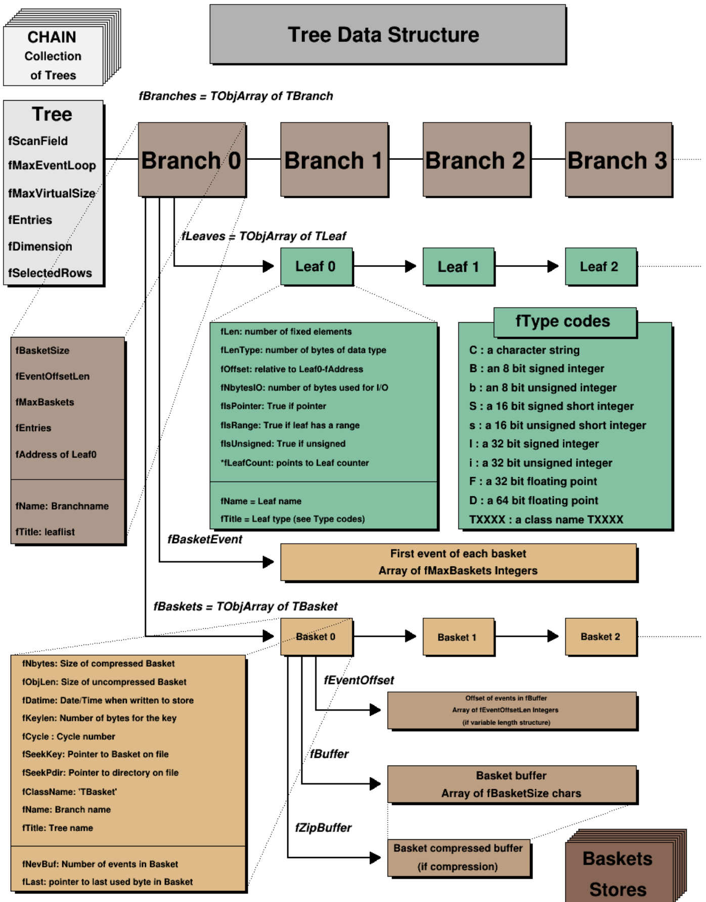
Figure 12.3: The TTree class
