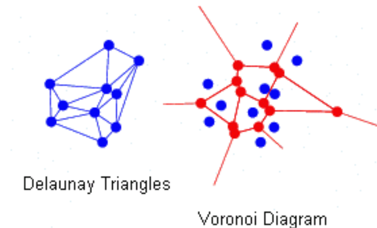
Figure 4.14: Delaunay triangles and Voronoi diagram
