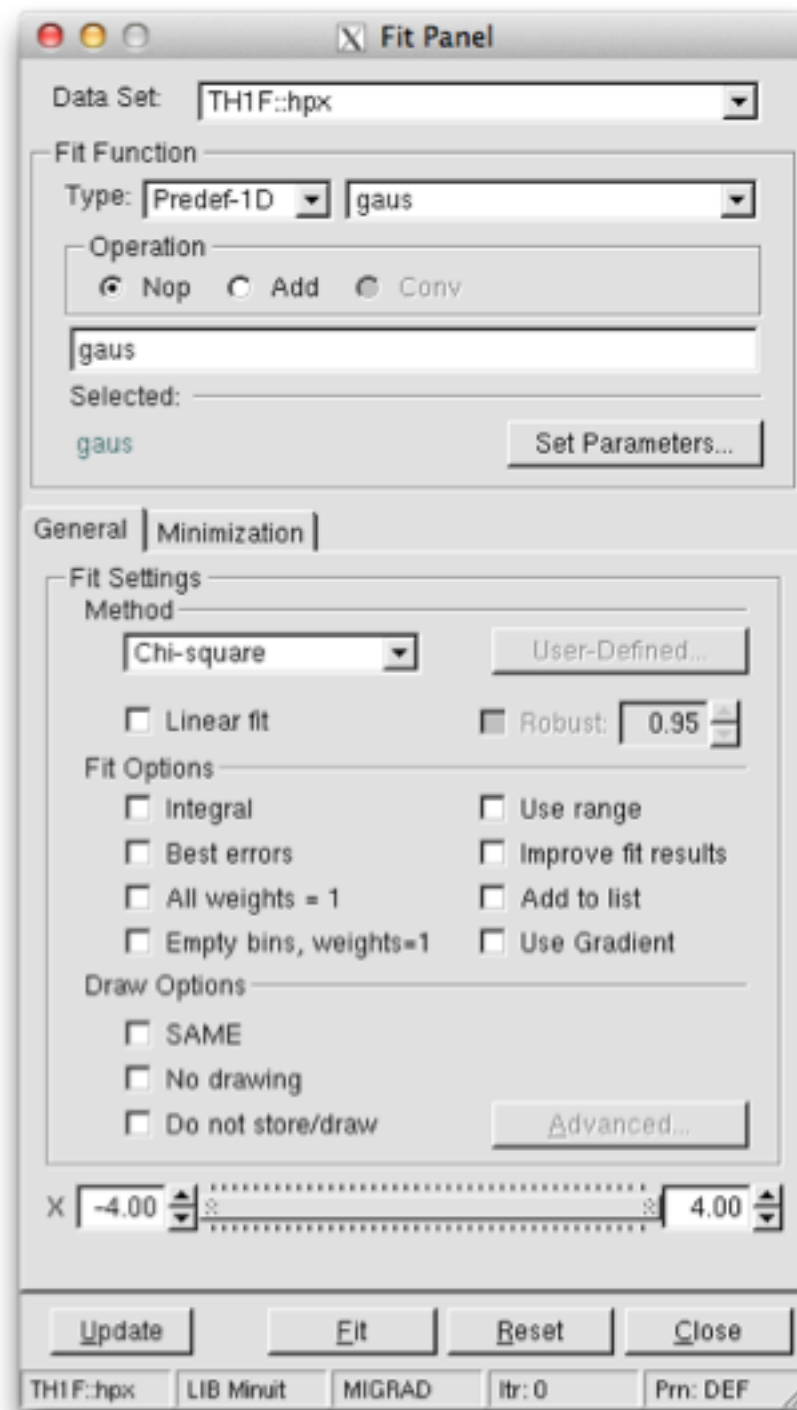
Figure 5.2: The Fit Panel
