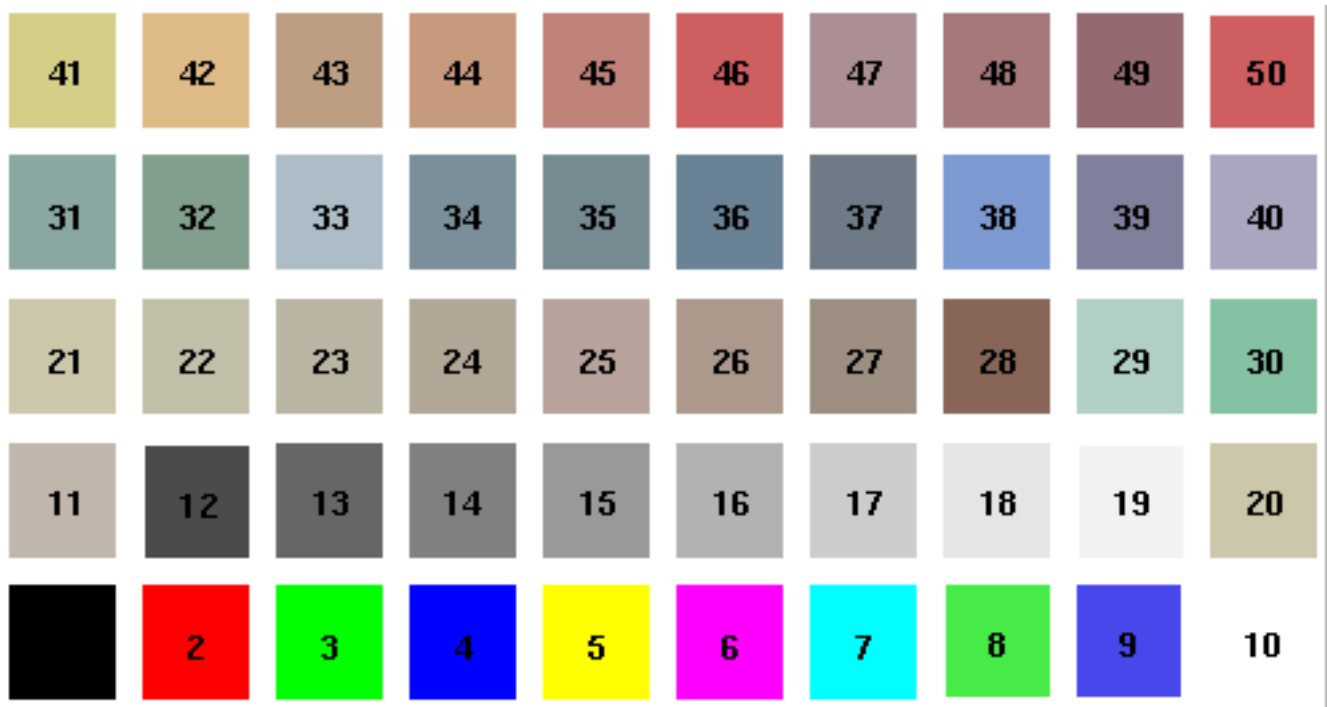
Figure 9.31: The basic ROOT colors
