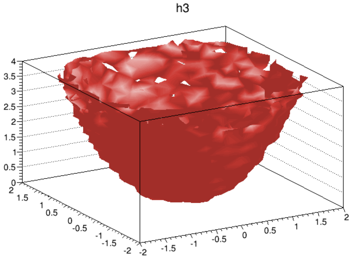
Figure 3.20: Iso surfaces
