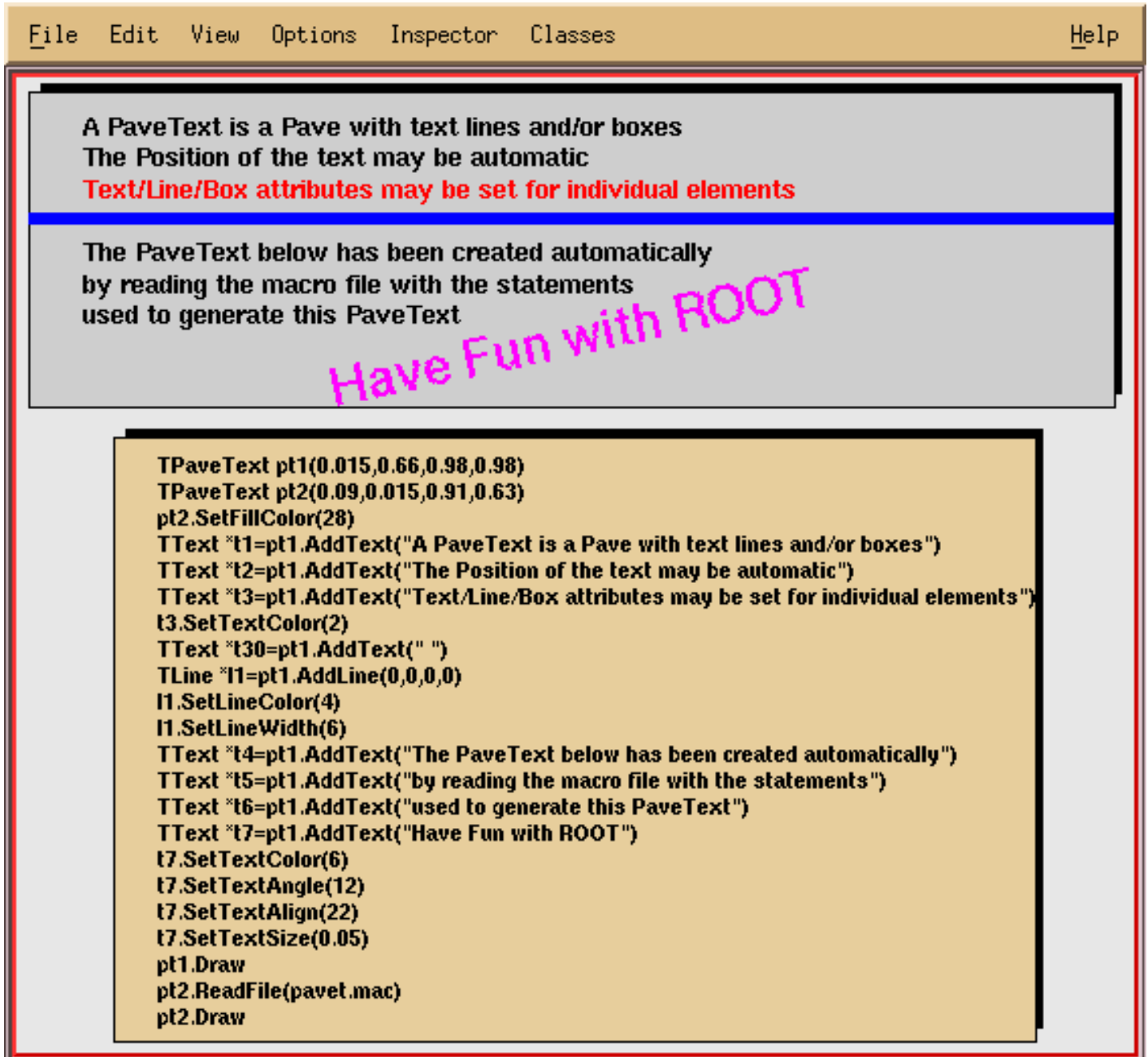
Figure 9.20: PaveText examples
