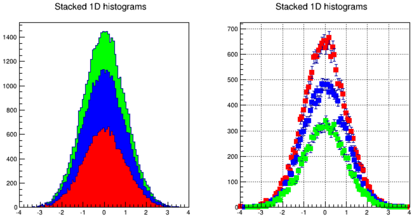
Figure 3.16: Stacked histograms
