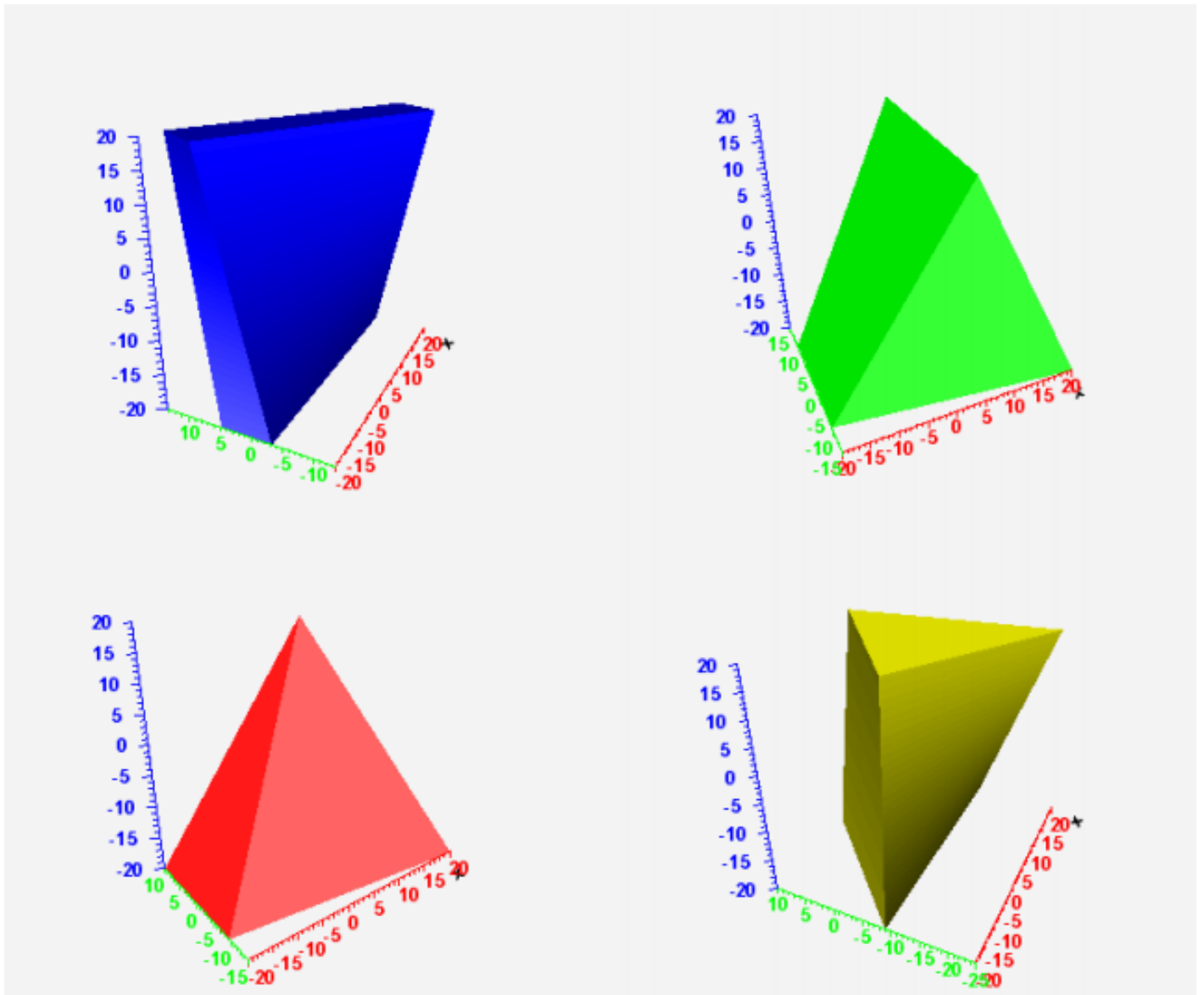
Figure 18.10: TGeoArb8 class
