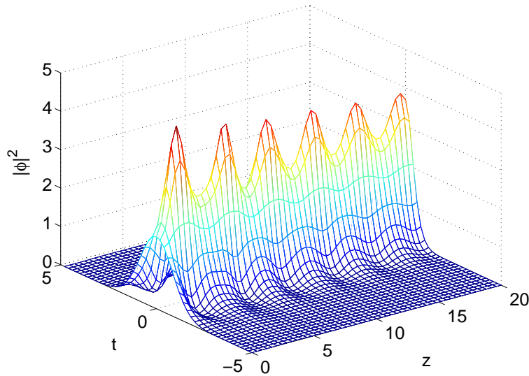
FIGURE 9.1: Results for nlse.xmDS
