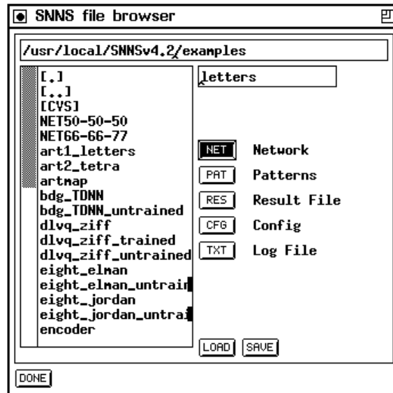
Figure 4.9: File Panel.
