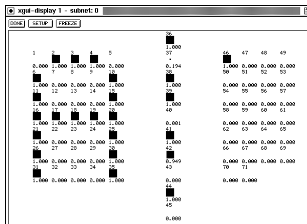
Figure 11.2: 2D-display
