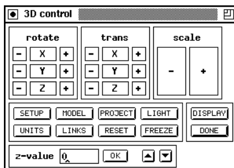
Figure 11.8: Control Panel
