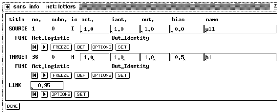
Figure 4.13: Info panel
