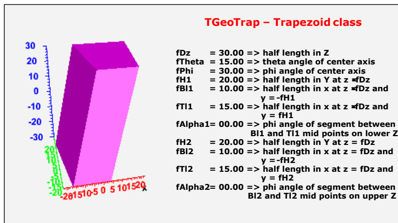
Figure 18-8 TGeoTrap Class
