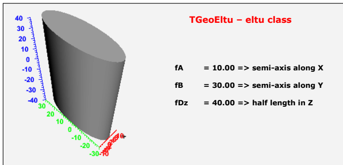
Figure 18-14 TGeoEltu Class
