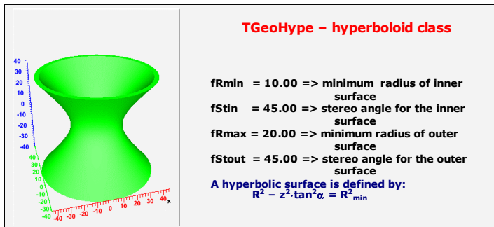
Figure 18-15 TGeoHype Class
