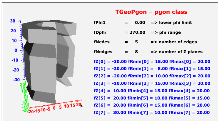
Figure 18-22 TGeoPgon Class
