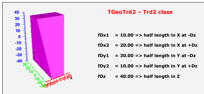
Figure 18-7 TGeoTrd2 class
