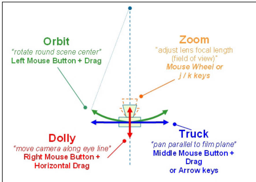
Figure 9-32 GL Viewer camera interactions
