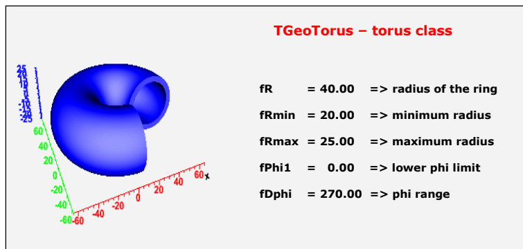
Figure 18-19 TGeoTorus Class
