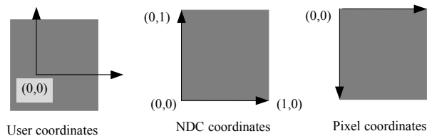
Figure 9-3 Pad coordinate systems
