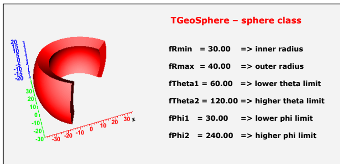
Figure 18-18 TGeoSphere Class
