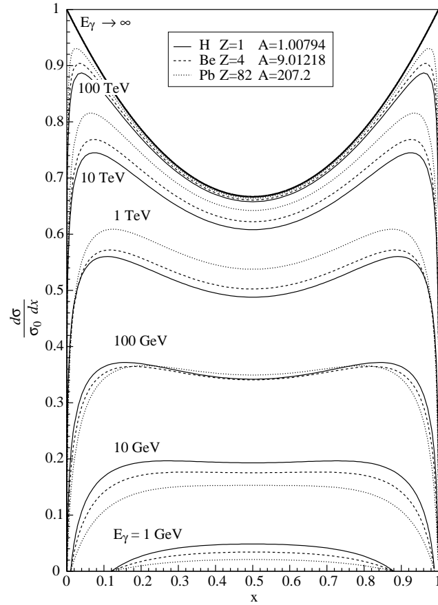
Figure 5.1: Normalized differential cross section for pair production as a function of x , the energy fraction of the photon energy carried by one of the leptons in the pair. The function is shown for three different elements, hydrogen, beryllium and lead, and for a wide range of photon energies.
