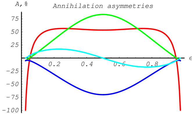
Figure 17.9: Annihilation differential cross section asymmetries in%. Red line corresponds to A_{ZZ}(\epsilon) , green line -A_{XX}(\epsilon) , blue line -A_{YY}(\epsilon) , lightblue line -A_{ZX}(\epsilon) . Kinetic energy of the incoming positron T_{k_1} = 10\text{MeV} .
