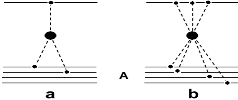
Figure 29.18: Possible enhanced diagrams of hA -interactions.
