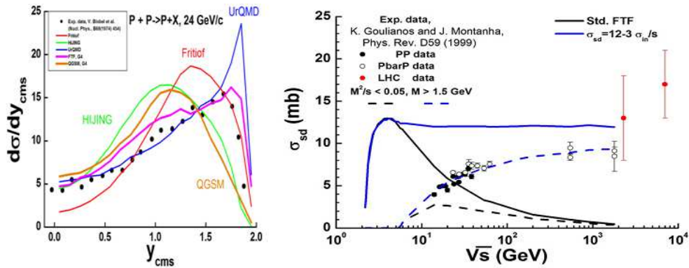
Figure 29.11: Left: inclusive spectrum of proton in pp -interactions at P_{lab} = 24 GeV/c. Points are experimental data [14], lines are model calculations. Right: single diffraction dissociation cross section in pp -interactions. Points are data gathered by K. Goulianos and J. Montanha [15]. Lines are FTF model calculations.
