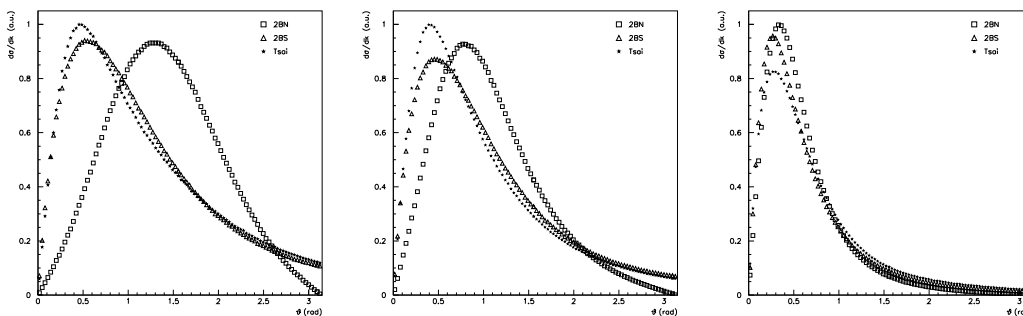
Figure 9.1: Comparison of polar angle distribution of bremsstrahlung photons ( k/T = 0.5 ) for 10 keV ( left ) and 100 keV ( middle ) and 500 keV ( right ) electrons in silver, obtained with Tsai, 2BS and 2BN generator
