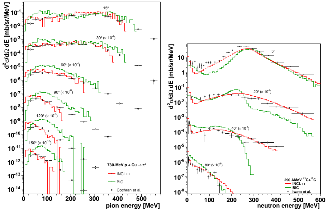
Figure 40.2: Left: double-differential cross sections for the production of charged pions in 730-MeV p+\text{Cu} . Right: double-differential cross sections for the production of neutrons in 290-AMeV ^{12}\text{C}+^{12}\text{C} . Predictions of the INCL++ and Binary-Cascade models are compared with experimental data from Refs. [5] and [6].
