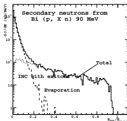
Figure 31.1: Secondary neutrons generated by Bertini INC with exitons and evaporation model.
