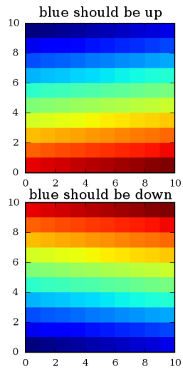
Figure 3.11: Controlling the image origin with the origin keyword argument to imshow and figimage ; see Listing 3.7.
