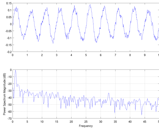
Figure 1.1: Colored noise signal and power spectrum generated with MATLAB™ as shown in Listing 1.1. Compare with matplotlib in Figure 1.2.
