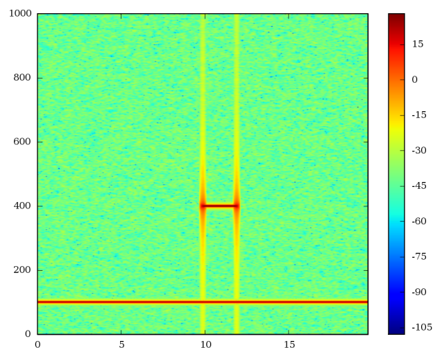
Figure 3.12: A spectrogram generated by Listing 3.8
