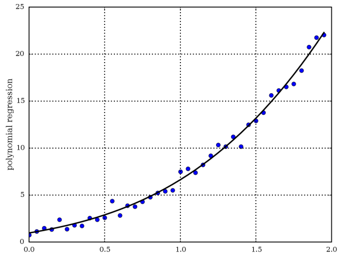
Figure 7.3: Estimating a best fit cubic for some random data; see Listing 7.3
