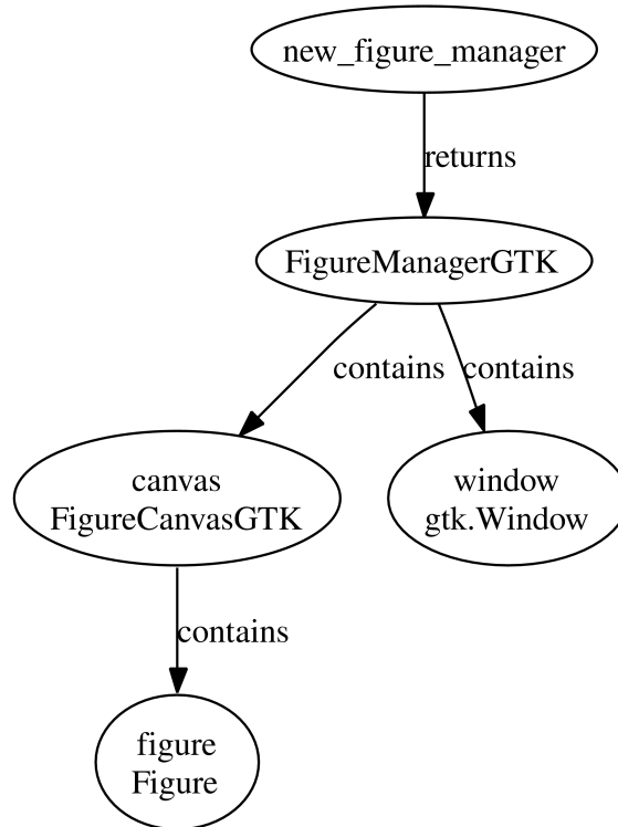
Figure 8.5: The pylab interface function new_figure_manager returns a backend dependent concrete implementation of matplotlib.backend_bases.FigureManagerBase , which contains the figure canvas and figure window. The attribute names are shown in lower case, and the backend dependent classes are shown in upper case. The standard attribute naming system allows the MATLAB™ interface to make calls across backends to the figure canvas and figure.
