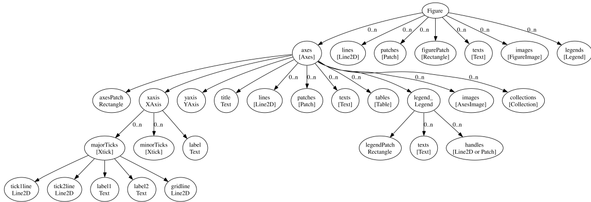
Figure 8.4: The Artist containment hierarchy. The top level Artist is the matplotlib.figure.Figure , which contains all of the other Artist instances. The attribute names are given in lower case, and the object type is listed below in upper case. If the attribute is a sequence, for example the figure contains a list of Axes, then the connecting edge is labeled 0..n and the object type is in square brackets to indicate a list, eg [Axes]. Some redundant information is omitted; for example, the yaxis contains the equivalent objects that the xaxis contains, the minorTicks have the same containment hierarchy as the majorTicks, and so on.
