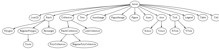
Figure 8.3: The matplotlib Artist hierarchy. The primitive Artists are the Patches, Line2D, Text, AxesImage, FigureImage and Collection classes. All other artists are composites of these. For example a Tick is comprised of a Line2D instance and a Text instance, which make up the tick line and tick label; the Axis is comprised of a list of Ticks and a Text axis label; see Figure 8.4.
