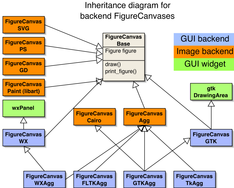
Figure 8.2: The inheritance diagram for The FigureCanvas hierarchy. The FigureCanvas is a backend dependent class which contains a figure instance. For GUI backends, the canvas should be a GUI widget embeddable in a GUI window. Some of the GUIs have backends with both native drawing and antigrain drawing (GTK/GTKAgg, WX/WX-Agg), which is readily achieved with multiple inheritance.
