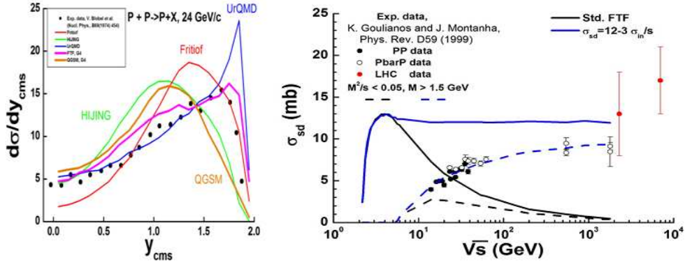
Figure 28.11: Left: inclusive spectrum of proton in pp-interactions at P_{\text{lab}} = 24 \text{ GeV}/c . Points are experimental data [14], lines are model calculations. Right: single diffraction dissociation cross section in pp-interactions. Points are data gathered by K. Goulios and J. Montanha [15]. Lines are FTF model calculations.
