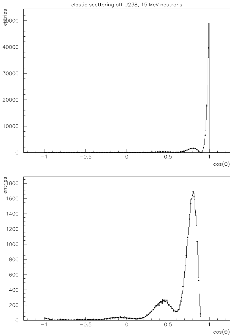
Figure 41.1: Comparison of data and Monte Carlo for the angular distribution of 15 MeV neutrons scattered elastically off Uranium ( ^{238}\text{U} ). The points are evaluated data, and the histogram is the Monte Carlo prediction. The lower plot excludes the forward peak, to better show the Fresnel structure of the angular distribution of the scattered neutron.
