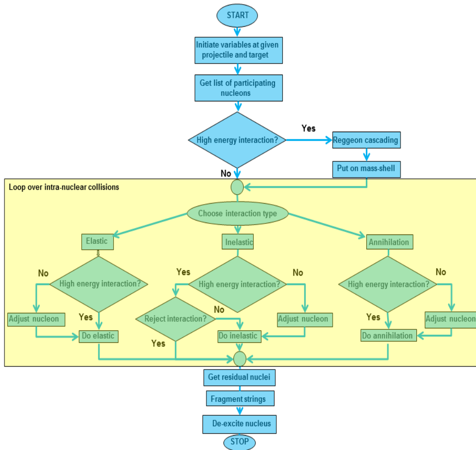
Figure 28.14: Flowchart of the FTF model.
