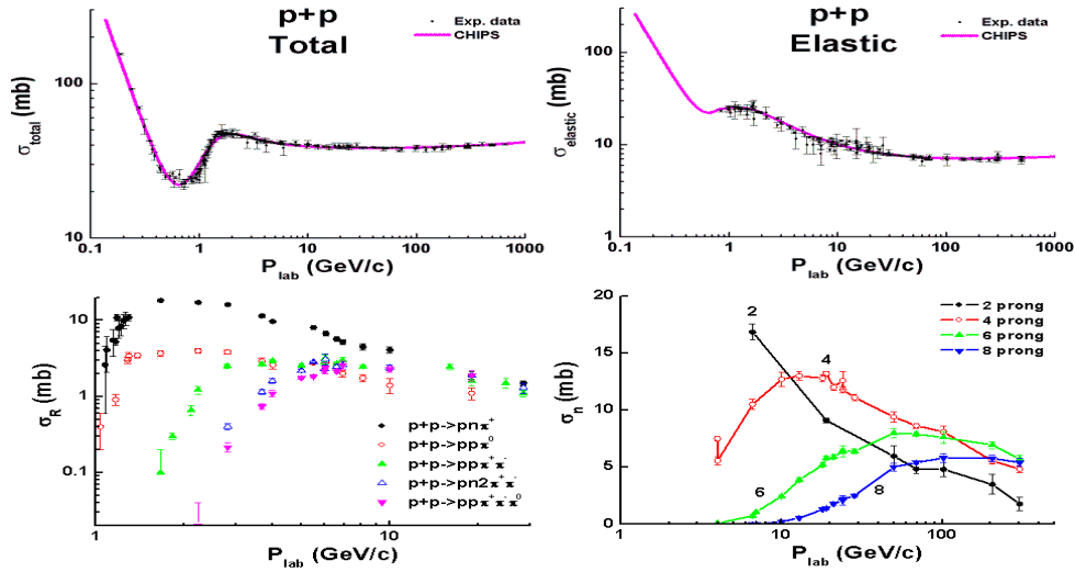
Figure 28.6: General properties of pp -interactions. Points are experimental data: data on total and elastic cross sections from PDG data-base [3], other data from [7].
