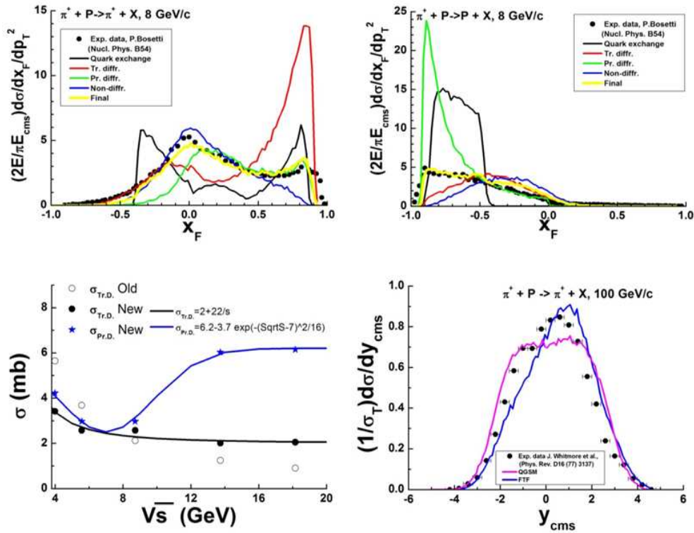
Figure 28.12: Upper figures: inclusive spectra of protons and \pi^+ -mesons in \pi^+p -interactions. Points are experimental data [16]. Lines represent the contributions of the various FTF processes calculated by assuming that the probability of each process is 100 %. Bottom left figure: diffraction dissociation cross sections obtained by tuning (points), and their description (lines) by the expression 28.19. Bottom right figure: rapidity spectrum of \pi^+ -mesons in \pi^+p -interactions at p_{\text{lab}} = 100 \text{ GeV}/c . Points are experimental data [17].
