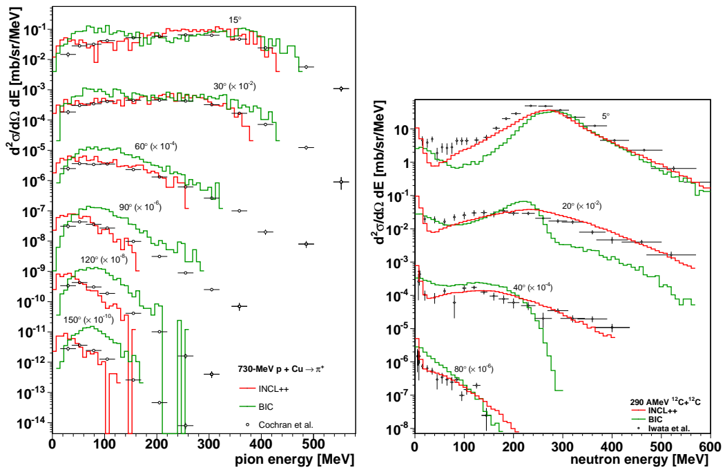
Figure 39.2: Left: double-differential cross sections for the production of charged pions in 730-MeV p+\text{Cu} . Right: double-differential cross sections for the production of neutrons in 290-AMeV ^{12}\text{C}+^{12}\text{C} . Predictions of the INCL++ and Binary-Cascade models are compared with experimental data from Refs. [5] and [6].
