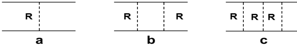
Figure 28.16: Nonenhanced diagrams of NN-scattering.
