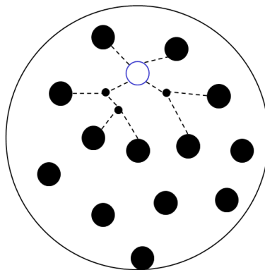
Figure 28.19: Reggeon "cascade" in hA -scattering.
