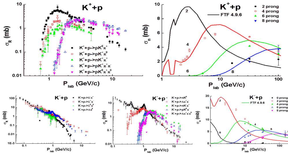
Figure 28.8: Reaction cross sections of Kp -interactions. Points are experimental data [8].
