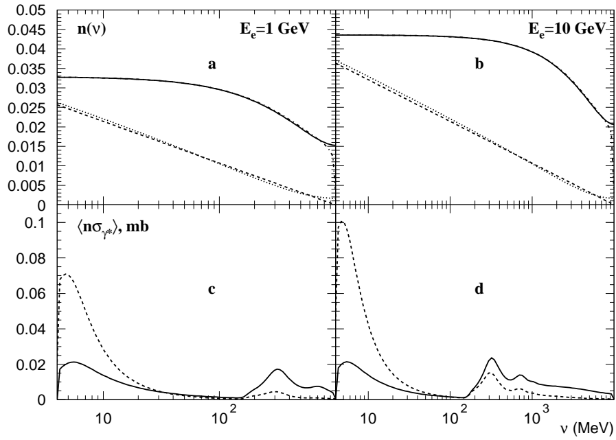
Figure 46.1: Relative contribution of equivalent photons with small Q^2 to the total “photon flux” for (a) 1 GeV electrons and (b) 10 GeV electrons. In figures (c) and (d) the equivalent photon distribution dn(\nu, Q^2) is multiplied by the photonuclear cross section \sigma_{\gamma^*}(K, Q^2) and integrated over Q^2 in two regions: the dashed lines are integrals over the low- Q^2 equivalent photons (under the dashed line in the first two figures), and the solid lines are integrals over the high- Q^2 equivalent photons (above the dashed lines in the first two figures).
