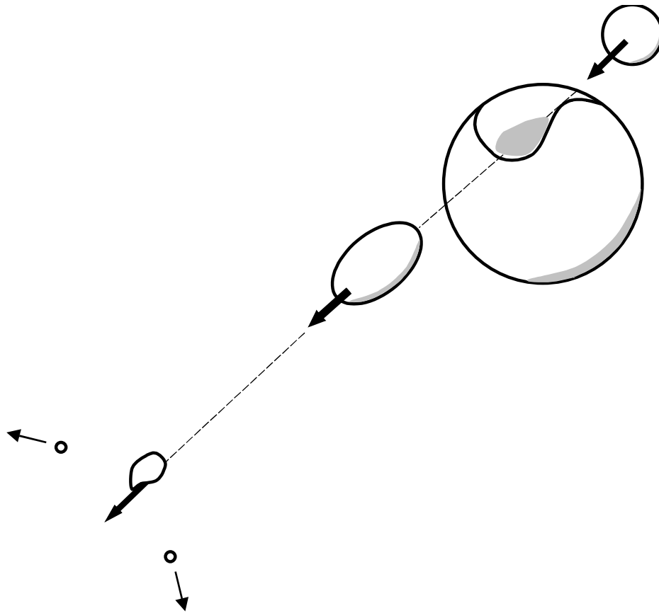
Figure 32.1: In the abrasion process, a fraction of the nucleons in the projectile and target nucleons interact to form a fireball region with a velocity between that of the projectile and the target. The remaining spectator nucleons in the projectile and target are not initially affected (although they do suffer change as a result of longer-term de-excitation).
