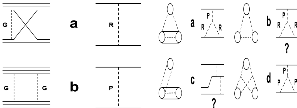
Figure 28.20: Diagrams of quark-gluon exchanges and corresponding reggeon diagrams for hadron-hadron interactions.
