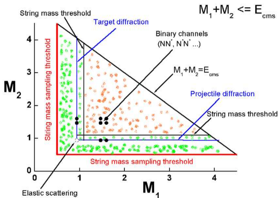
Figure 28.2: Diagram of the final states of hadron-hadron interactions.
