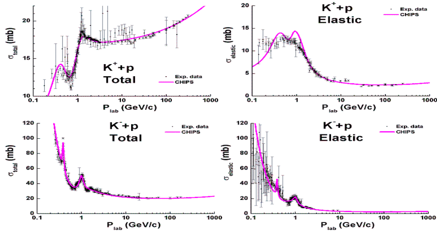
Figure 28.7: Total and elastic cross sections of Kp -interactions. Points are experimental data from PDG data-base [3].
