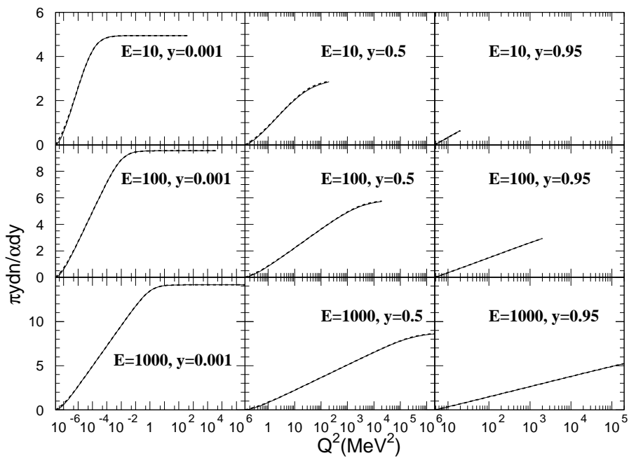
Figure 46.2: Integrals of Q^2 spectra of virtual photons for three energies 10 MeV, 100 MeV, and 1 GeV at y = 0.001 , y = 0.5 , and y = 0.95 . The solid line corresponds to Eq.(46.13) and the dashed line (which almost everywhere coincides with the solid line) corresponds to Eq.(46.13).
