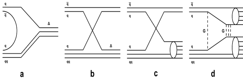
Figure 28.4: Quark flow diagrams of \pi N -interactions.
