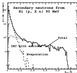
Figure 29.1: Secondary neutrons generated by Bertini INC with exitons and evaporation model.
