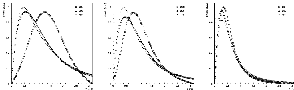
Figure 9.3: Comparison of polar angle distribution of bremsstrahlung photons ( k/T = 0.5 ) for 10 keV ( left ) and 100 keV ( middle ) and 500 keV ( right ) electrons in silver, obtained with Tsai, 2BS and 2BN generator
