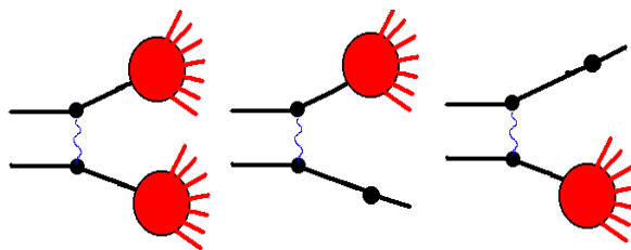
Figure 28.1: Non-diffractive and diffractive interactions considered in the Fritiof model.
