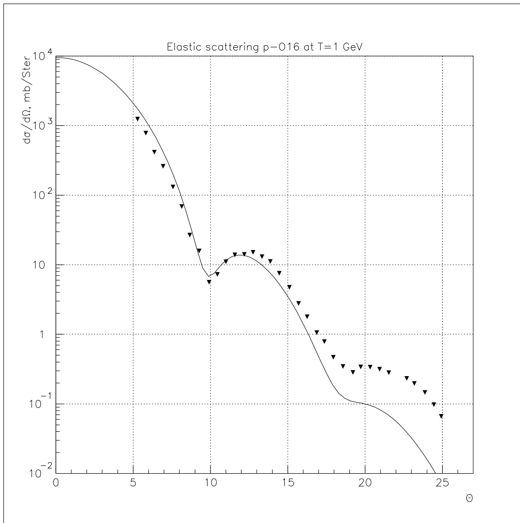
Figure 25.4: Elastic proton scattering on 16 O at 1 GeV
