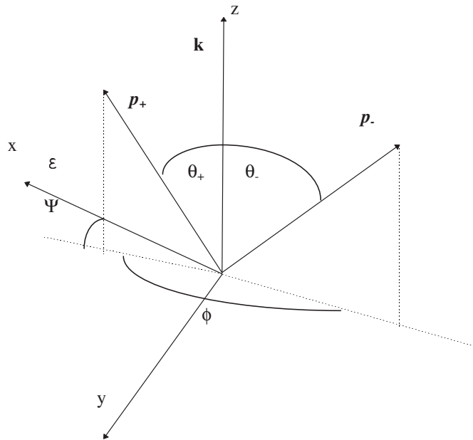
Figure 9.1: Angles occurring in the pair creation
