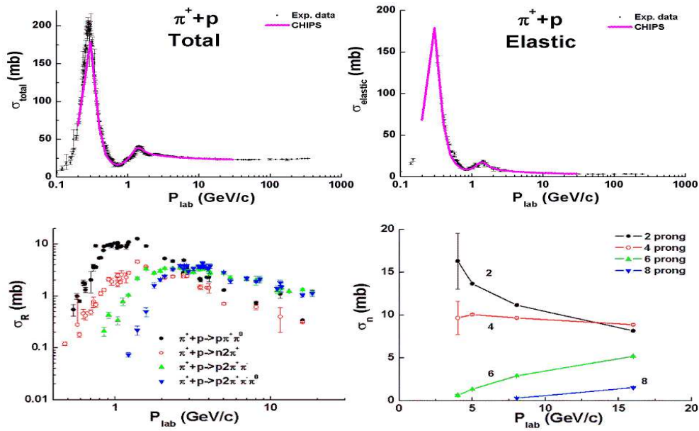
Figure 28.5: General properties of \pi^+p -interactions. Points are experimental data: data on total and elastic cross sections from PDG data-base [3], other data from [4].
