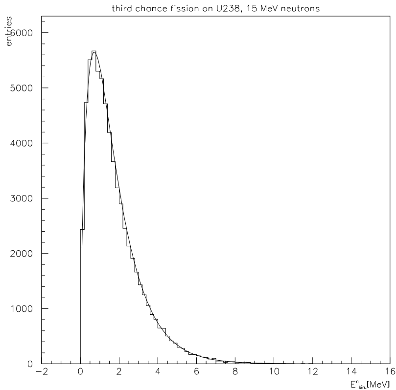
Figure 41.3: Comparison of data and Monte Carlo for fission neutron energy distributions for induced fission by 15 MeV neutrons on Uranium ( ^{238}\text{U} ). The curve represents evaluated data and the histogram is the Monte Carlo prediction.
