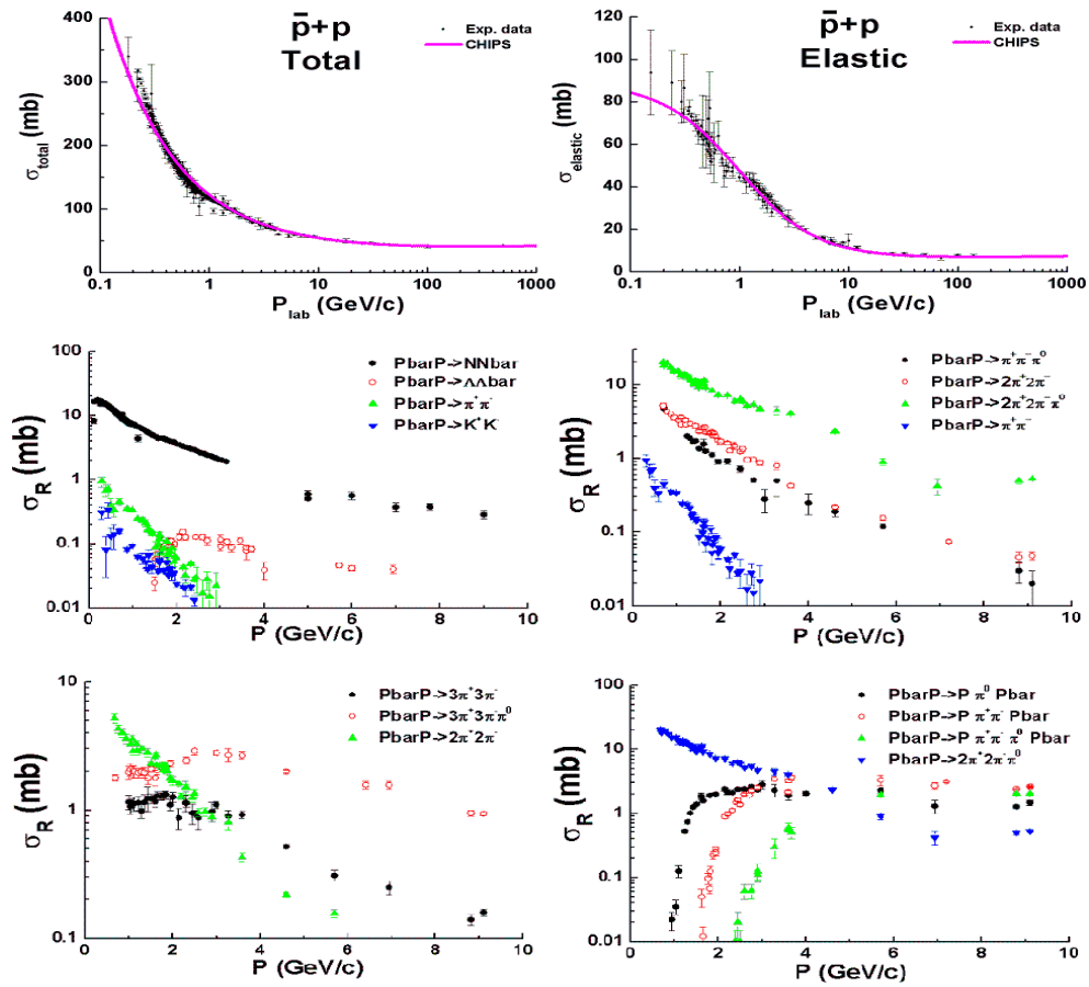
Figure 28.9: General properties of p\bar{p} -interactions. Points are experimental data: data on total and elastic cross sections from PDG data-base [3], other data from [7].
