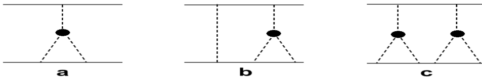
Figure 28.17: Simplest enhanced diagrams of NN-scattering.
