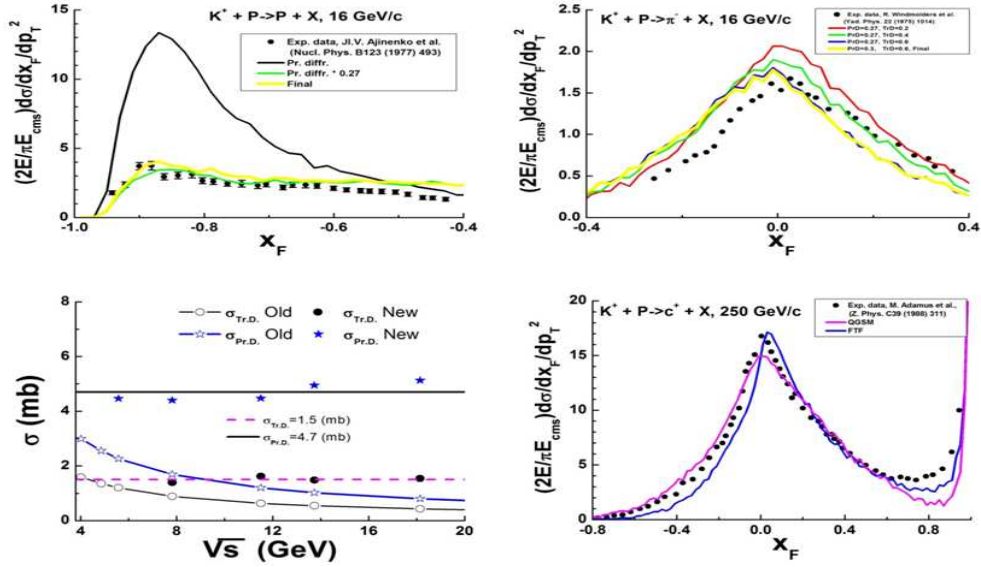
Figure 28.13: Upper figures: inclusive spectra of protons and \pi^- -mesons in Kp -interactions. Points are experimental data [18]. Lines are FTF calculations. Bottom left figure: diffraction dissociation cross sections obtained by tuning (points), and their description (lines) by the expression 28.20. Bottom right figure: x_F spectrum of positive charged particles in Kp -interactions at p_{\text{lab}} = 250 GeV/c. Points are experimental data [17], lines are model calculations.
