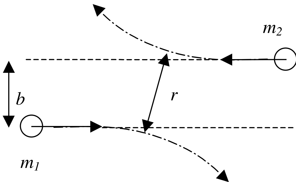
Figure 32.2: Illustration clarifying impact parameter in the far-field ( b ) and actual impact parameter ( r ).
