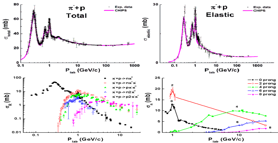
Figure 28.3: General properties of \pi^-p -interactions. Points are experimental data: data on total and elastic cross sections from PDG data-base [3], other data from [4].
