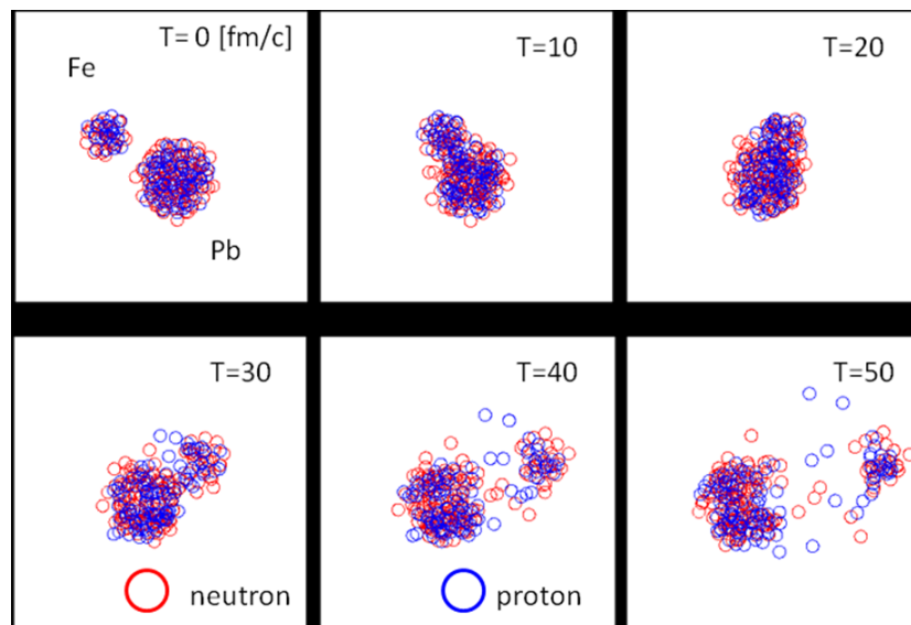
Figure 31.1: Time evolution of reaction of 290 MeV/n Fe on Pb in position space. Red and Blue circle represents neutron and proton respectively. Full scale of each panel is 50 fm.
