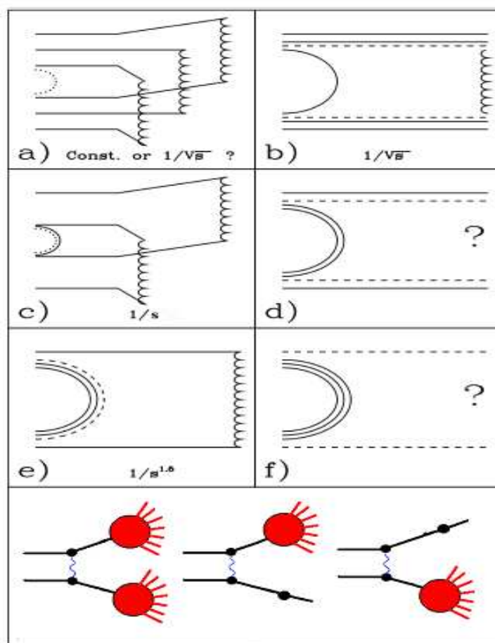
Figure 28.10: Quark flow diagrams of \bar{p}p -interactions.
