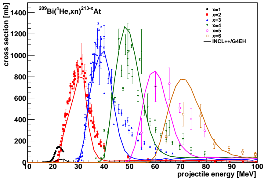
Figure 39.3: Excitation functions for (\alpha, xn) cross sections on ^{209}\text{Bi} . The predictions of INCL++-G4ExcitationHandler are represented by the solid line and are compared to experimental data [7, 8, 9, 10, 11, 12, 13, 14, 15].
