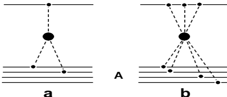
Figure 28.18: Possible enhanced diagrams of hA -interactions.
