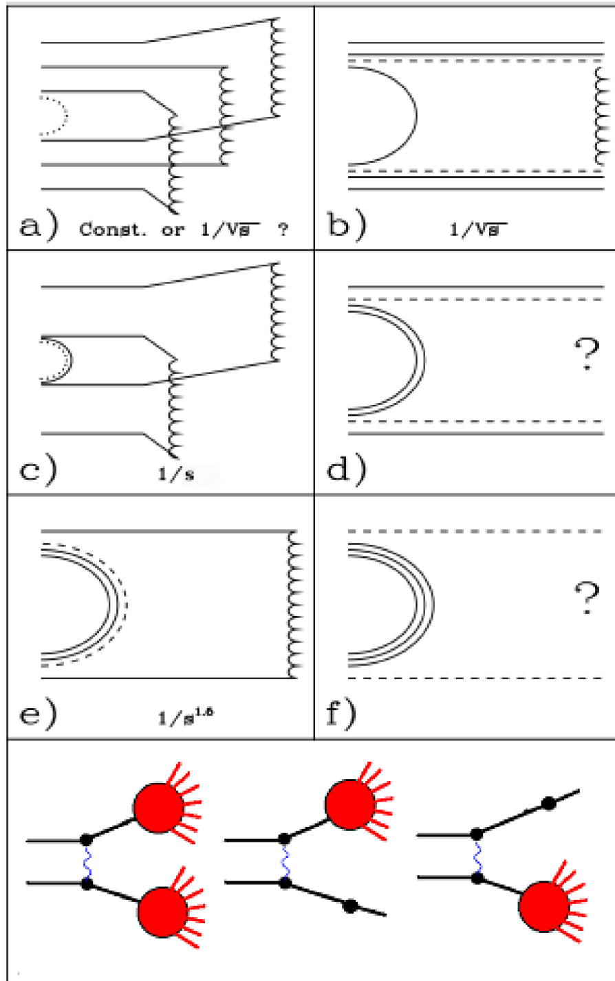
Fig. 3.11: Quark flow diagrams of p\bar{p} -interactions.
