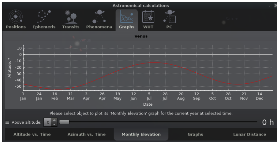
Figure 4.33: Astronomical Calculations (AstroCalc): Graphs / Monthly Elevation
