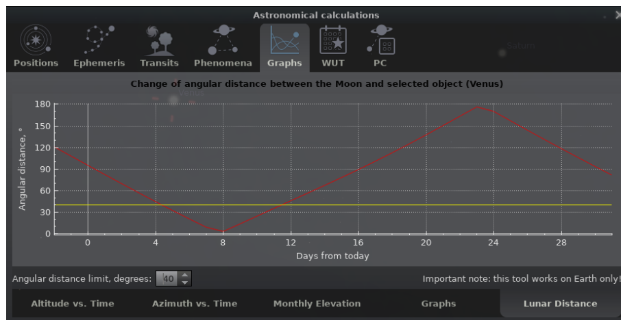
Figure 4.35: Astronomical Calculations (AstroCalc): Graphs / Lunar Distance
