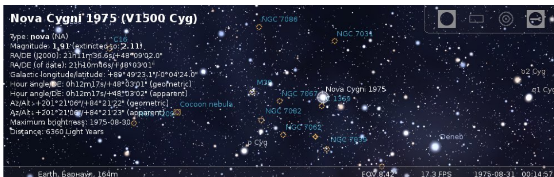
Figure 13.1: Nova Cygni 1975 (also known as V1500 Cyg )
