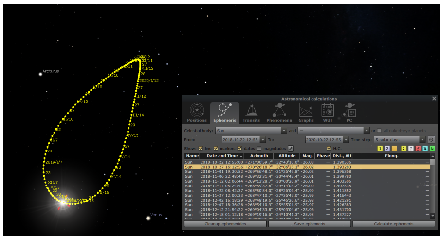
Figure 4.27: Astronomical Calculations (AstroCalc): Analemma on Mars
