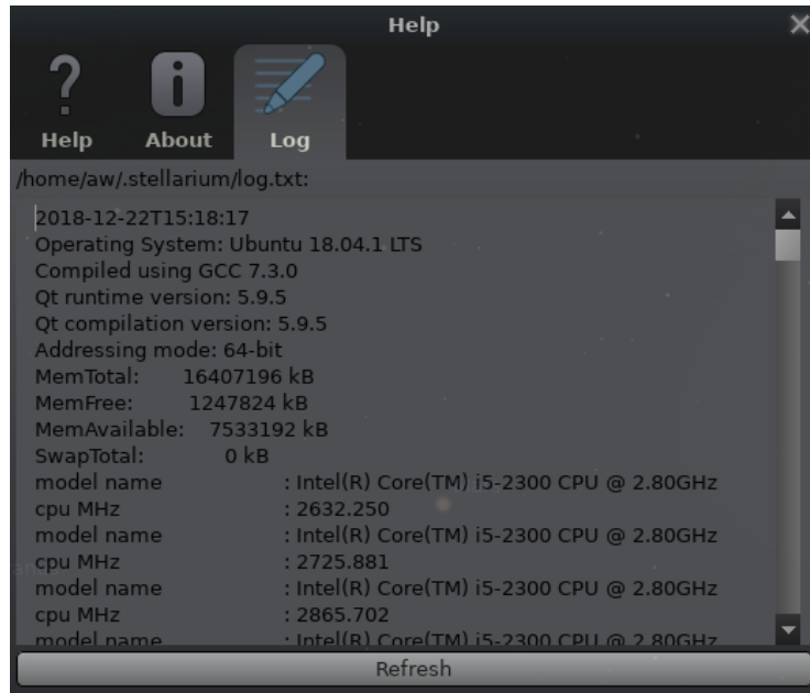
Figure 4.41: Help Window: Logfile
