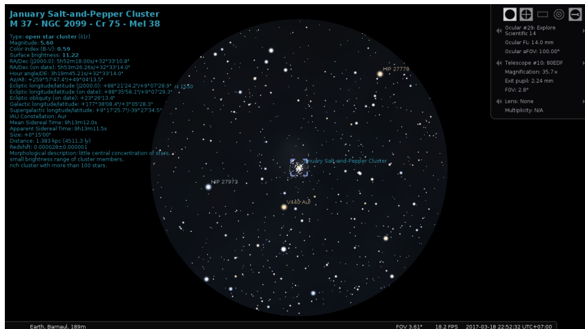
Figure 15.9: The M37 cluster through a Celestron 80 mm EDF with Explore Scientific 14 mm eyepiece.
