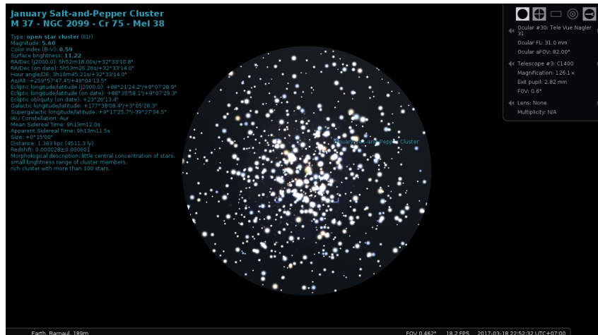
Figure 15.10: The M37 cluster through a Celestron C1400 with Tele Vue Nagler 31 mm eyepiece.
