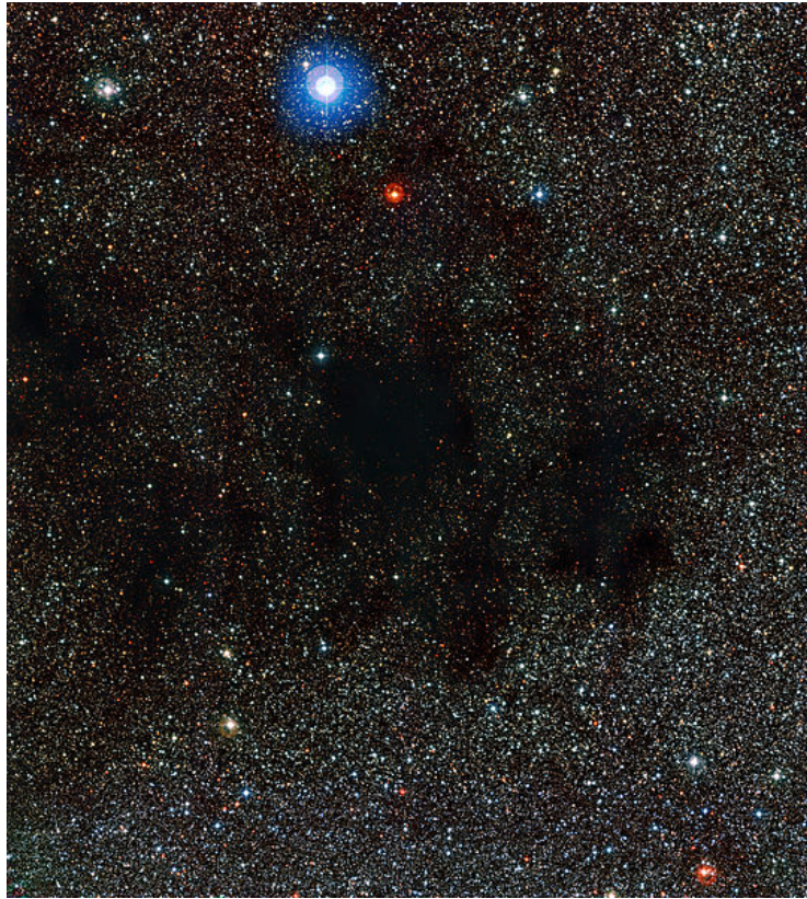
Figure 19.3: The Coalsack Nebula taken by the Wide Field Imager on the MPG/ESO 2.2-metre telescope. Credit: ESO.
