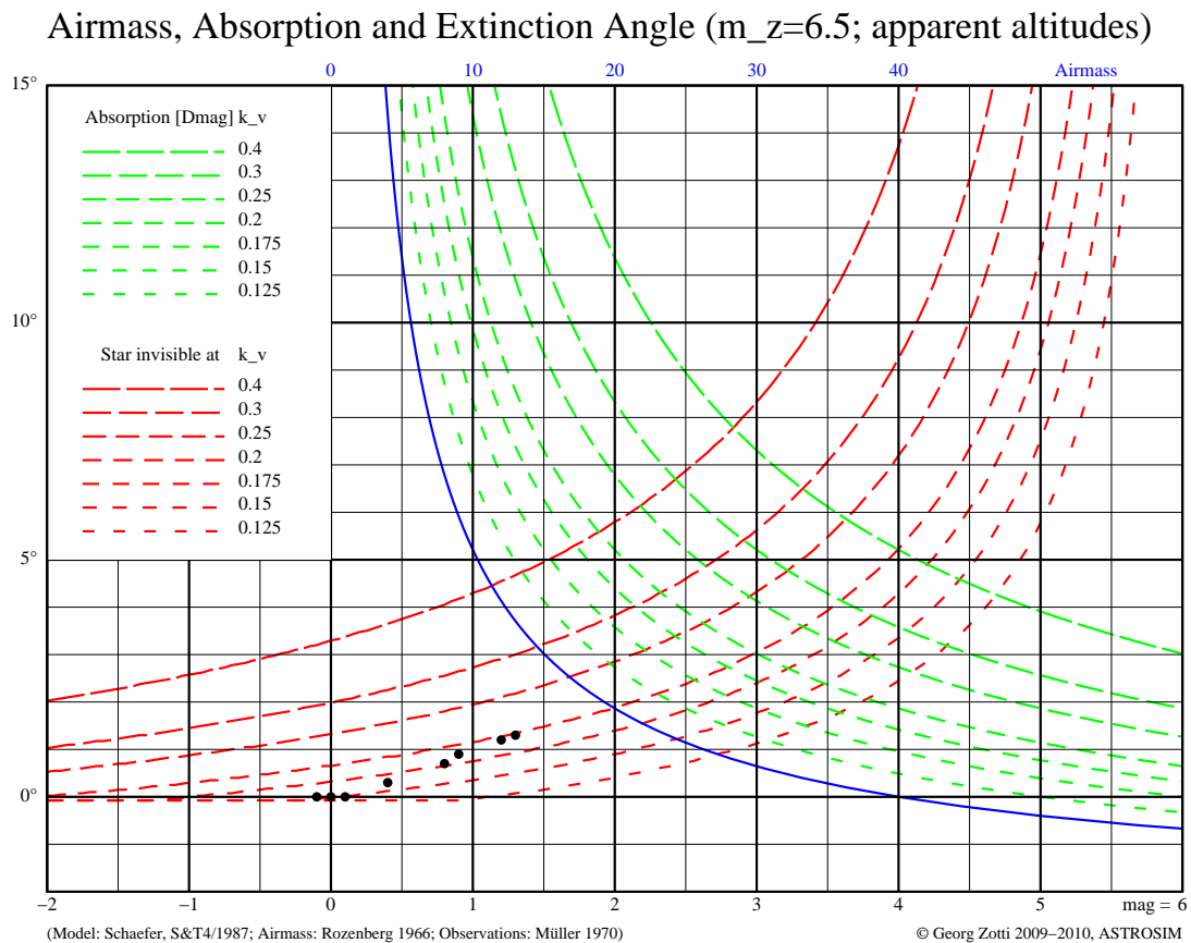
Figure 18.5: Airmass and Extinction. The figure shows Airmass (blue) along the line of sight in the altitude labeled on the left side. The green curves show how many magnitudes an object is dimmed down, depending on extinction factor k (called k_v in the figure). The red curves indicate at which altitude a star of given magnitude can be seen with good eyesight, again depending on k . The black dots are observed values found in the literature.
