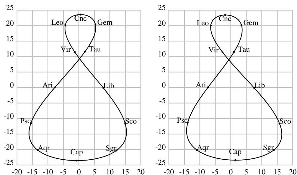
Figure 12.1: Figure-8 plots for Equation of Time, for years 1000 (left) and 2000 (right). These plots, often found on sundials, link solar declination (vertical axis) and its deviation at mean noon from the meridian, in minutes. Labeled dots indicate when the sun entered the respective Zodiacal sign ( 30^\circ section of the ecliptic). Figures by Georg Zotti.
