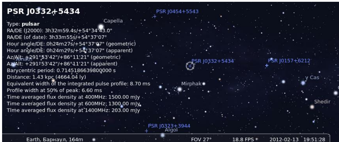
Figure 13.5: PSR J0332-5434
