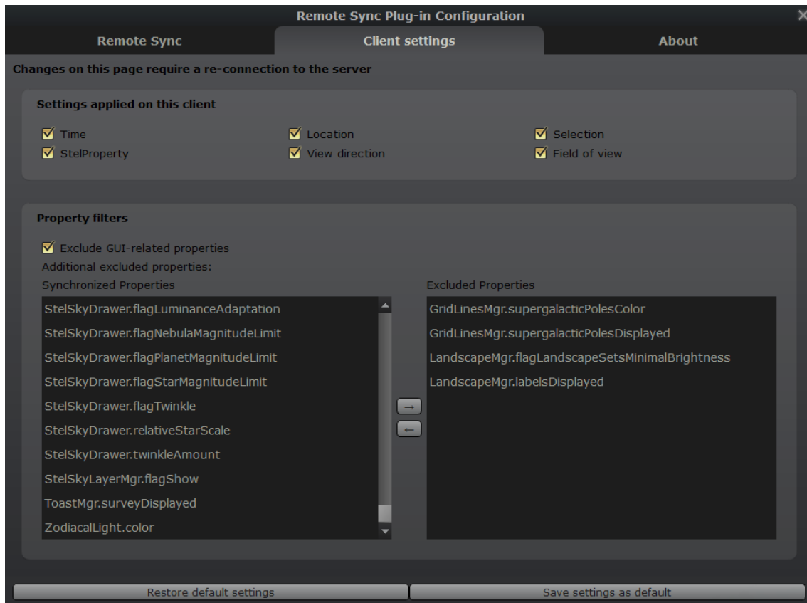
Figure 12.5: RemoteSync client settings window
