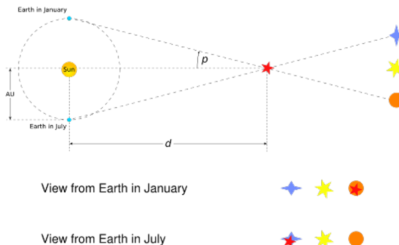
Figure 17.7: Stellar Parallax
